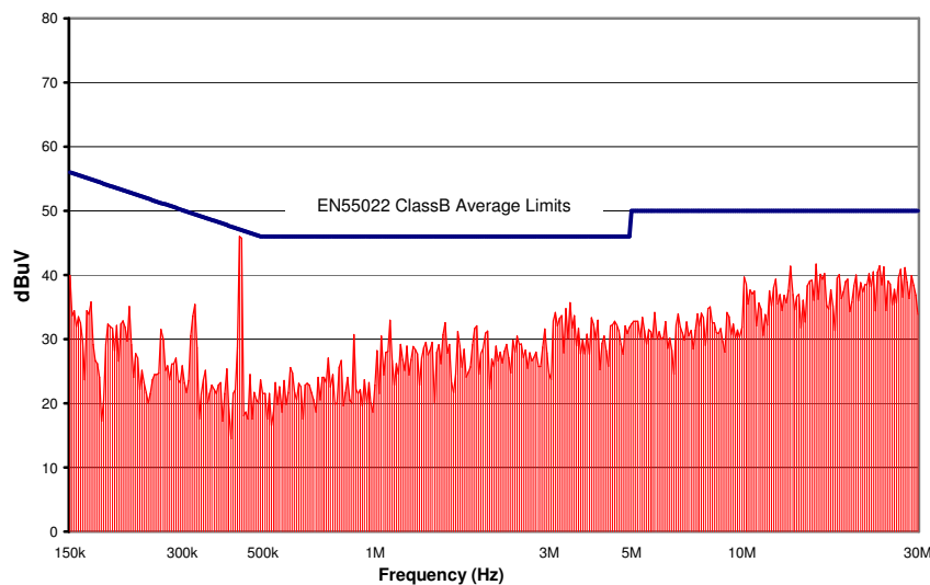
Figure 20. CP40_1233018 Conducted Emissions using above specified input filter. Vin = 24V, Full Resistive Load
