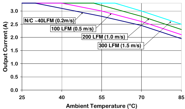
Figure 3. Output Current Derating vs Ambient Temperature & Airflow (Open Frame module) Vin = 24 V (airflow from pin 1 to pin 2)
