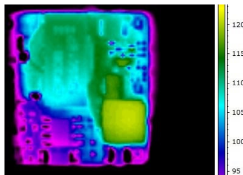
Figure 6. Thermal Image of CP40_1233018 3.3A output, 55C Ambient, 200lfm airflow, Vin = 24V, T max = 125°C
