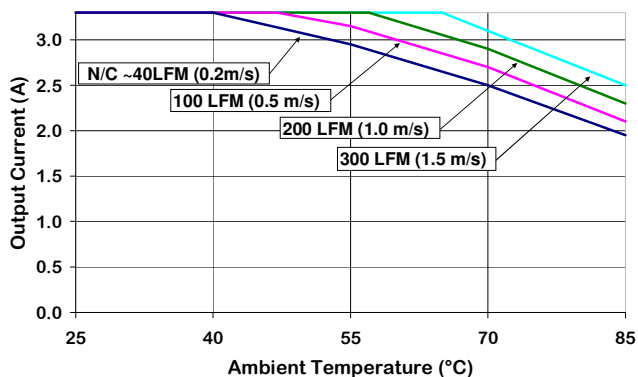
Figure 5. Output Current Derating vs Ambient Temperature & Airflow (Encapsulated module) Vin = 12V, 24V
