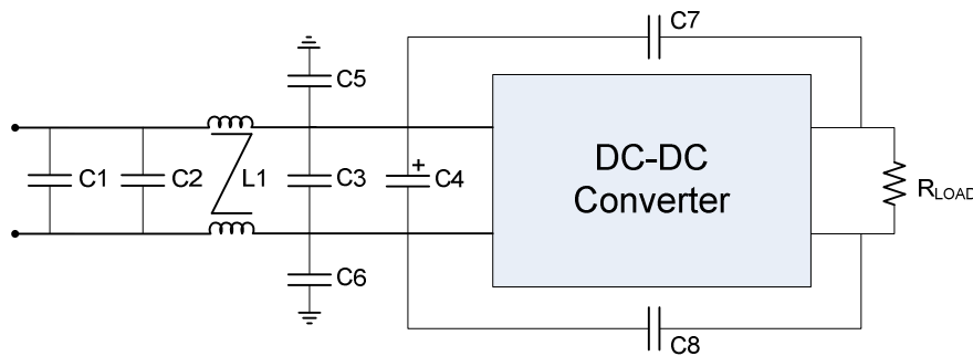
Figure 19. EMI Filter
